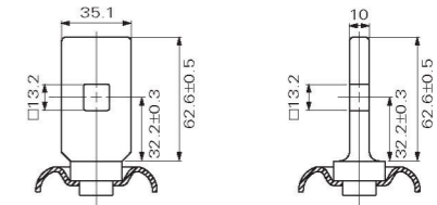
K1 Flange Fitting
